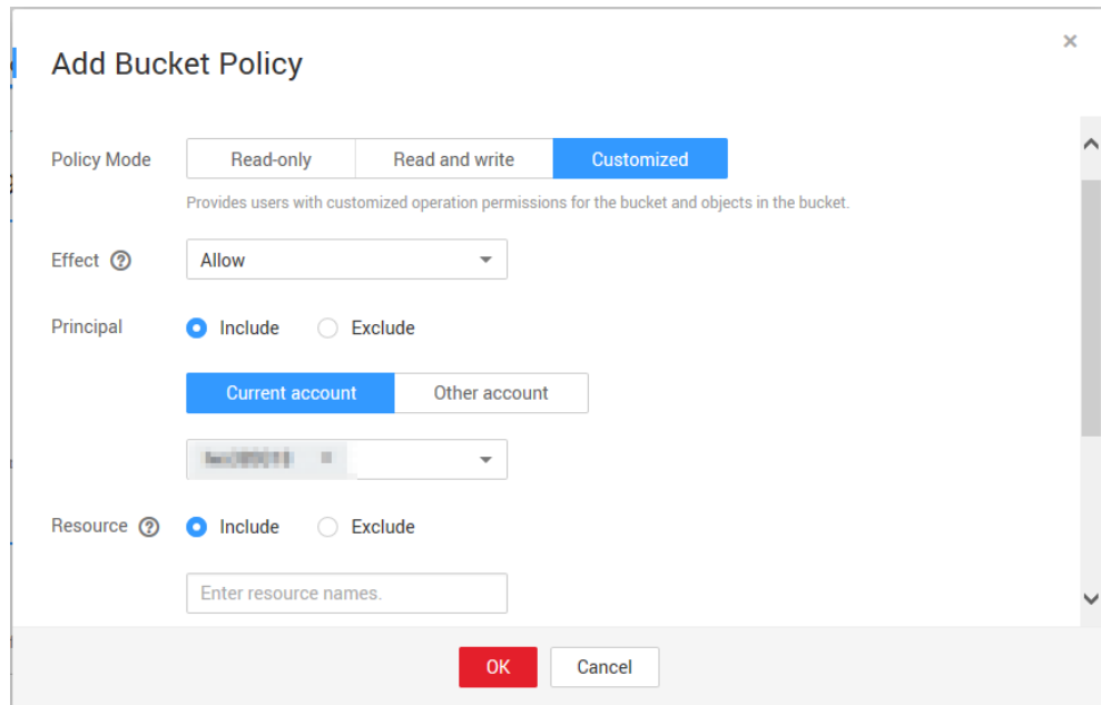
Figure 6-4 Adding a bucket policy
